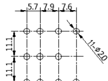
侧面法兰外壳(C1) Side flange cover(C1) MR20-1C/2C/3C-C1
